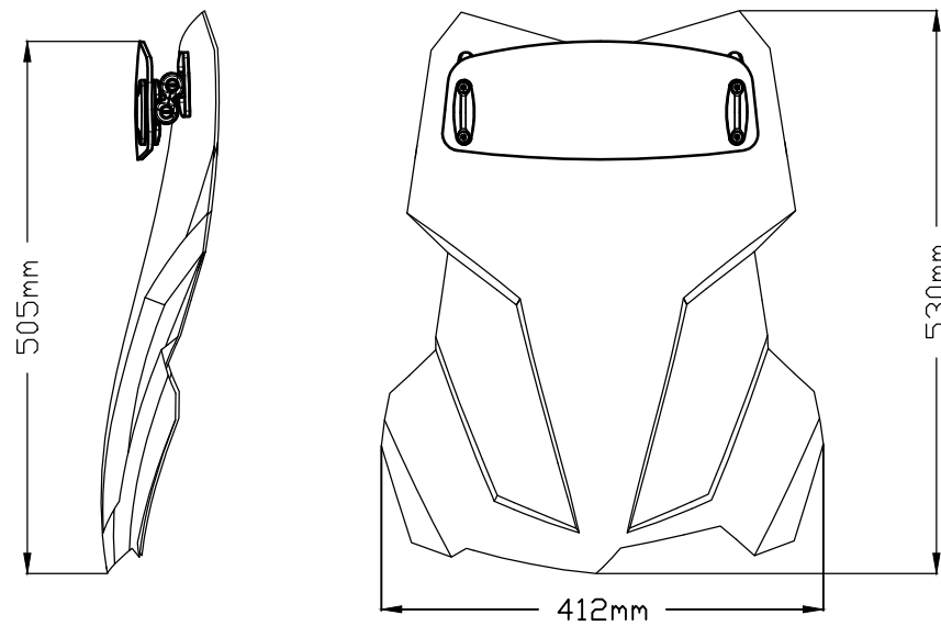
TOURING SCREEN WITH VISOR AT LOWER POSITION
