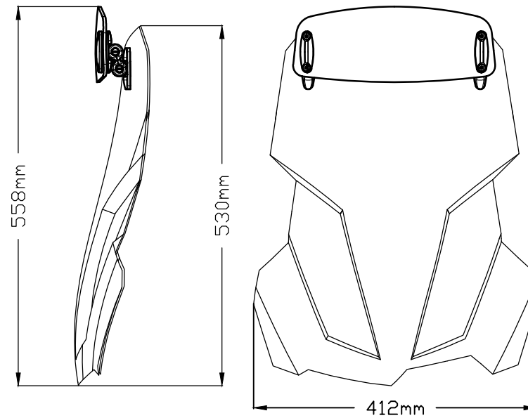
TOURING SCREEN WITH VISOR AT LOWER POSITION
