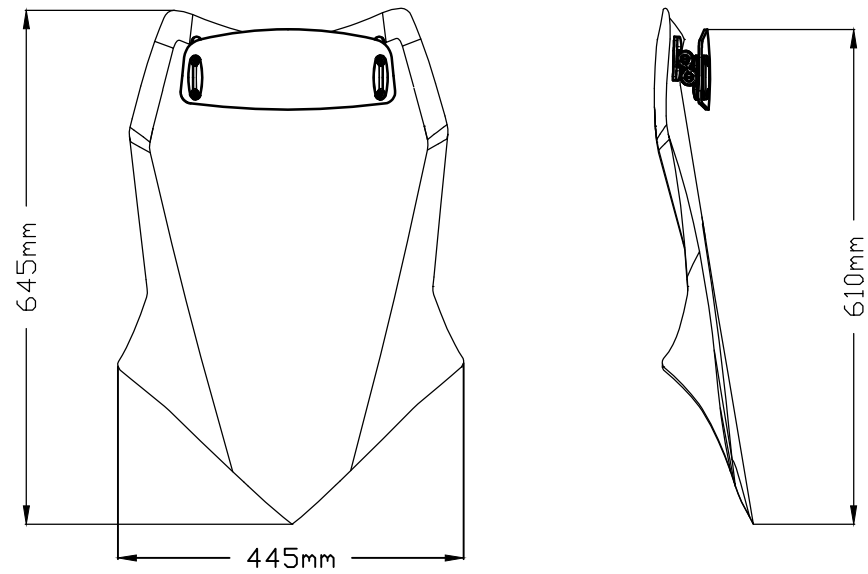
TOURING SCREEN WITH VISOR AT UPPER POSITION
