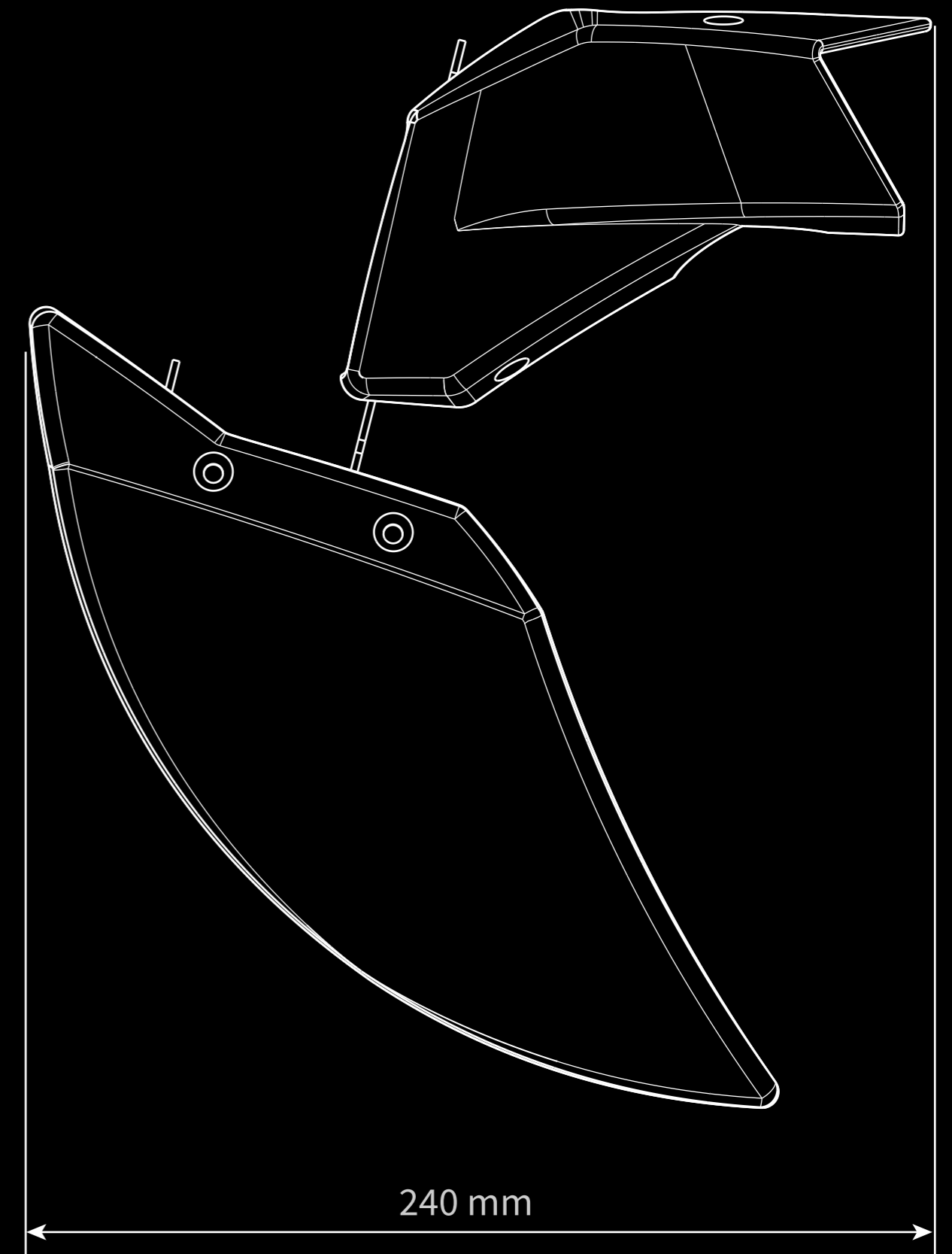
RIGHT BRAKE COOLER
